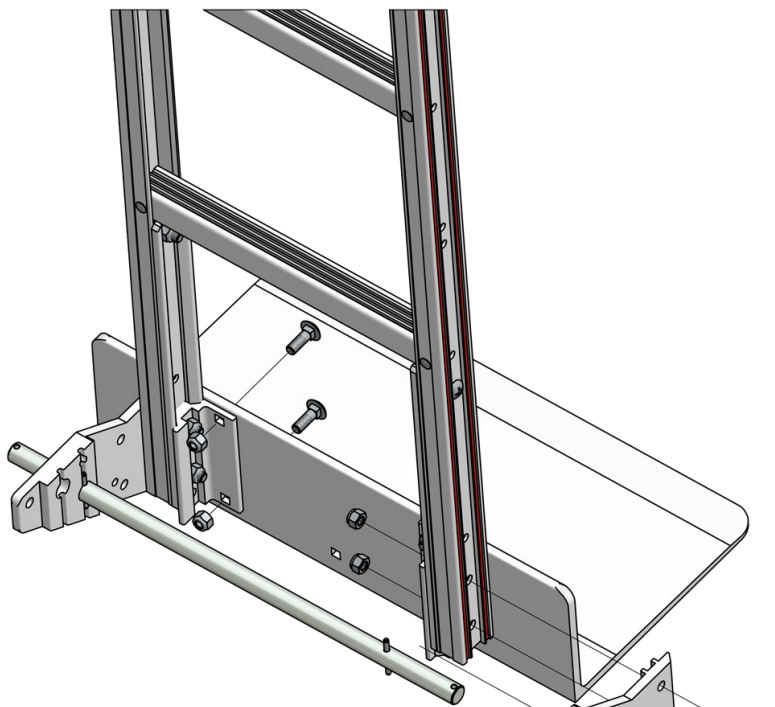
Forward mount nose plate with mounting brackets and 8" wheel axle location shown
